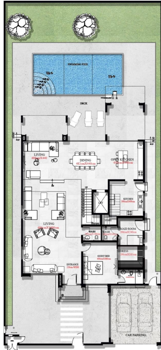
VILLA 53- GROUND FLOOR
