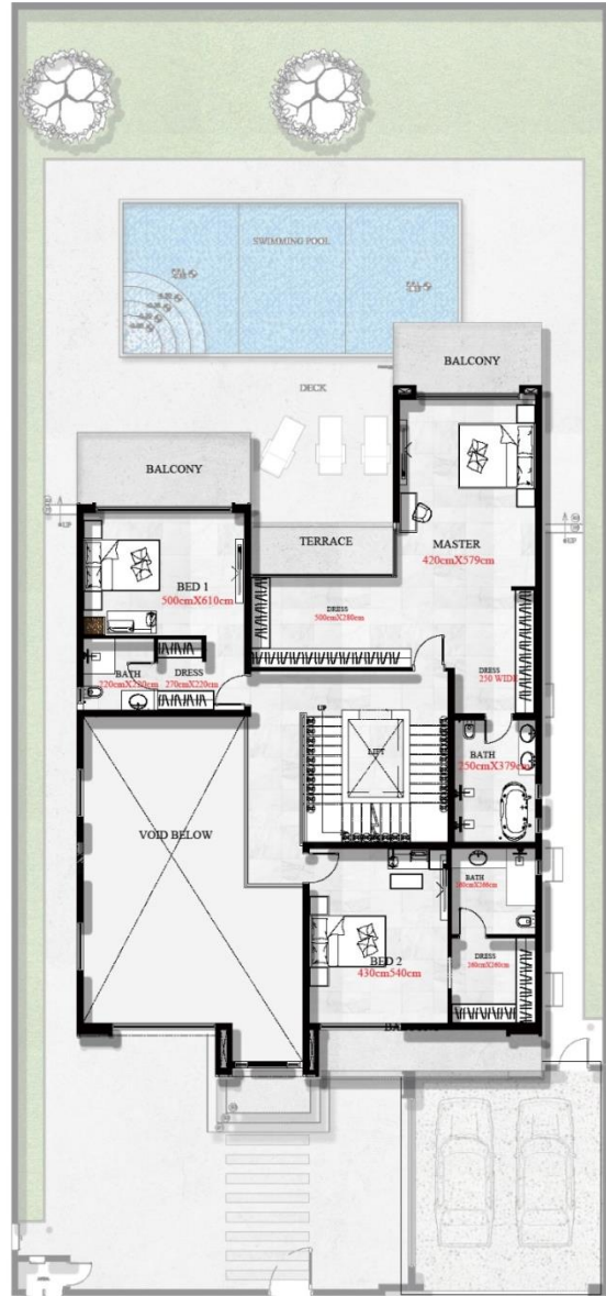
VILLA 53- FIRST FLOOR
